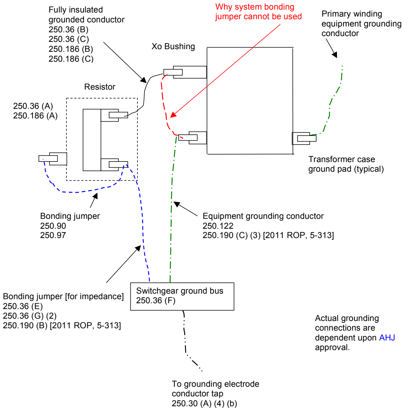
7.2.13. Figure – Power Transformer – Outside Building – Resistance Ground [No Line-to-Neutral Loads]
